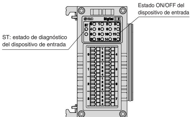
EX600-DX□F
